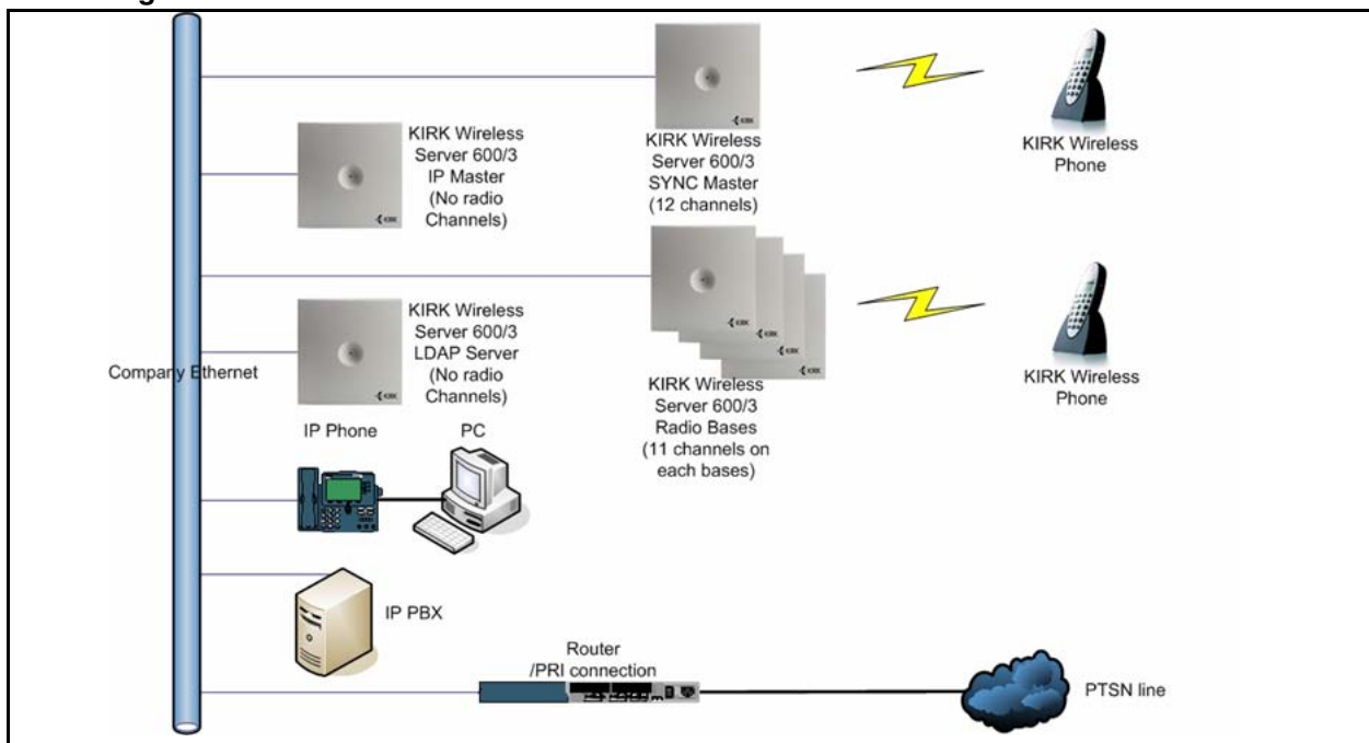
Figure 76 KWS600v3 Multi-cell installation with LDAP Server
